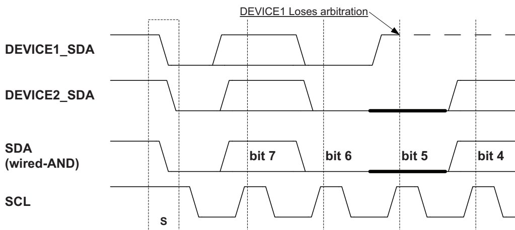
Figure 21-9. TWI arbitration.
