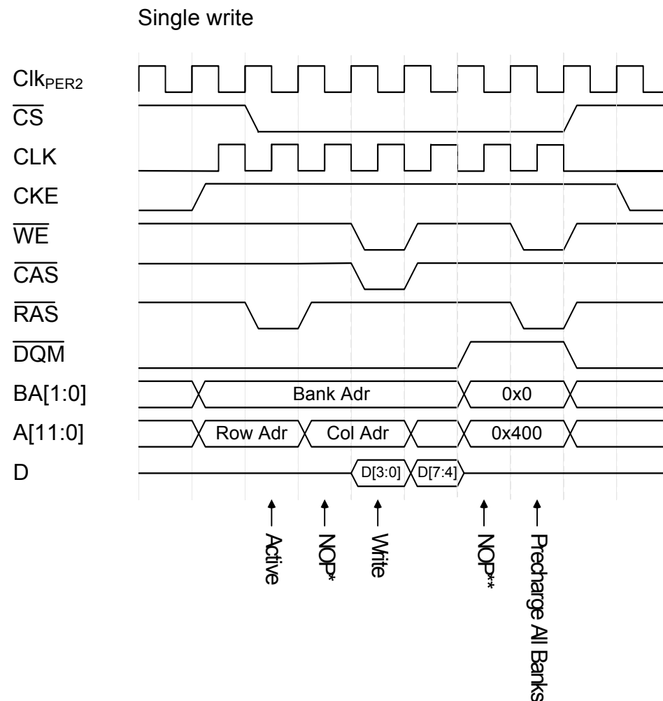
Figure 36-20. Single write
